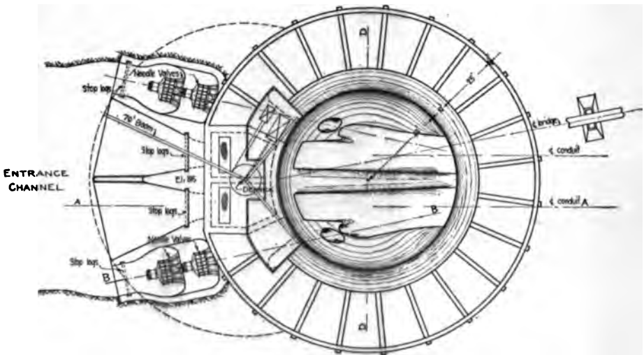
FIG. 50.—Outlet works for the proposed Dublin dam. The gates control the water of the small summer floods and for the Columbus water supply. In great floods, the outlet is automatic.
